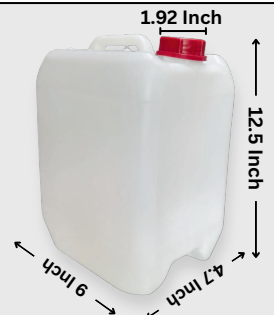
Jerry Can Milky White Capacity: 10 Ltr Weight: 560g (±10g) Colors: Blue, Natural White
