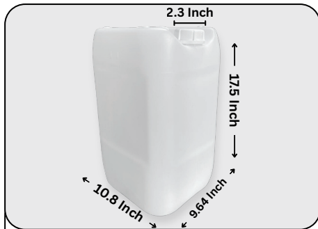
Jerry Can Natural White Capacity: 25 Ltr Weight: 1270g (±10g) Colors: Blue, Milky White
